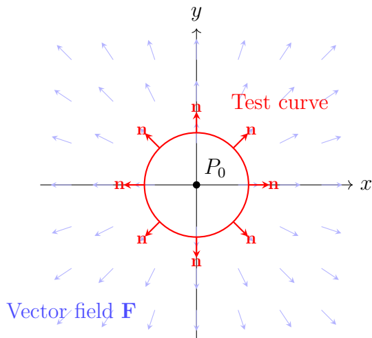
Figure 5.20: To measure divergence at point P_0 , we examine how much the vector field \mathbf{F} flows across a small test curve (red). The outward unit normal vectors \mathbf{n} help us measure the net outward flow.
