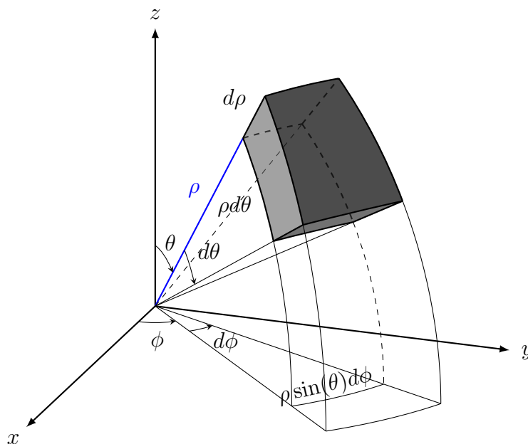
Figure 4.25: Representation of a volume element in spherical coordinates (\rho, \phi, \theta) , where \rho is the radial distance, \phi is the azimuthal angle in the xy -plane, and \theta is the polar angle from the z -axis. The volume element is defined by \rho^2 \sin \theta d\rho d\phi d\theta , illustrating the differential components d\rho , \rho d\theta , and \rho \sin \theta d\phi .
