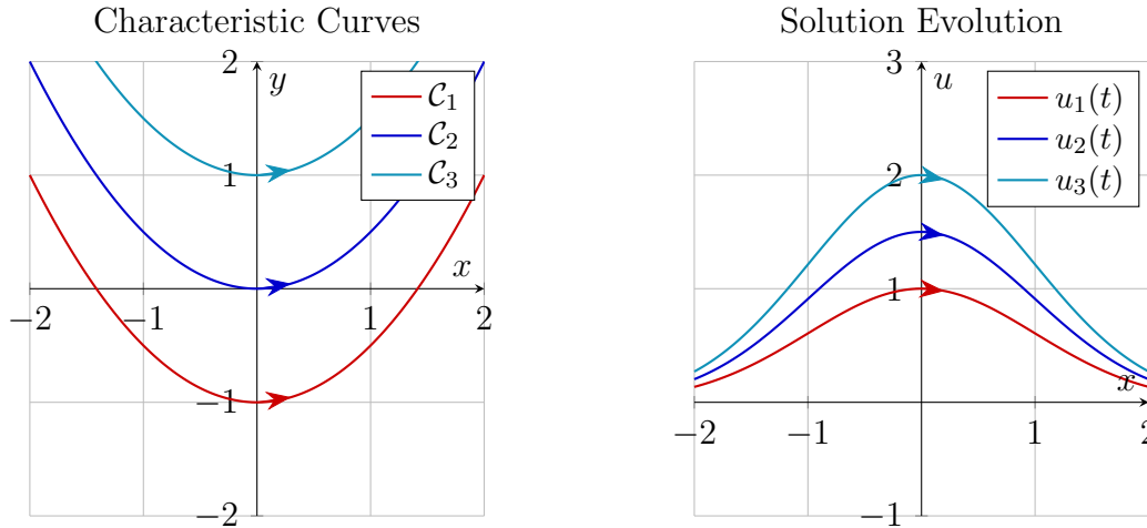
Figure 6.4: Geometric visualization of the method of characteristics. Left: Characteristic curves in the xy -plane showing the paths along which information propagates. Right: Evolution of the solution u along different characteristics, with matching colors indicating correspondence between paths and solutions. Each characteristic curve C_i determines the evolution of its corresponding solution u_i(t) .
