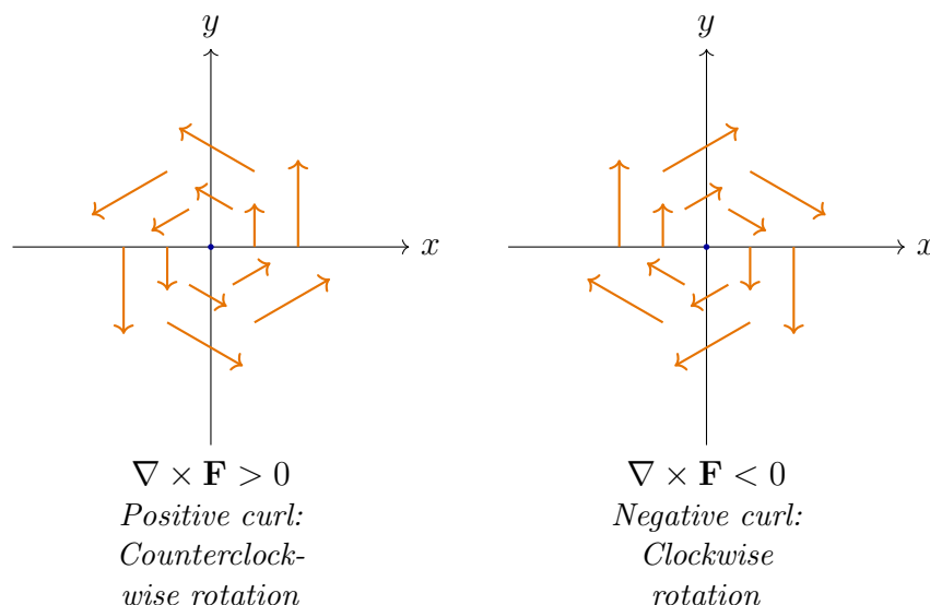
Figure 5.18: Patterns of curl in vector fields. Left: Positive curl ( \nabla \times \mathbf{F} > 0 ) corresponds to counterclockwise rotation. Right: Negative curl ( \nabla \times \mathbf{F} < 0 ) corresponds to clockwise rotation. The direction and magnitude of the curl quantify the rotational tendency of the field at a given point. When we say the curl is positive or negative in this case, we are referring to the \mathbf{k} component.
