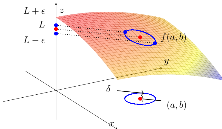
Figure 3.13: 3D plot with a \delta -circle, center point (a, b) , a transparent surface, f(a, b) , the circle plotted on the surface, and the corresponding points L , L + \epsilon , and L - \epsilon on the z -axis connected to their corresponding surface points.
