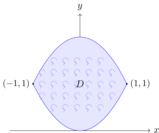
Figure 5.14: The basin region D bounded by y = x^2 and y = 2 - x^2 . Blue arrows indicate local vorticity patterns, demonstrating the symmetric flow structure about the vertical axis. This visualization helps us understand why the total vorticity integrates to 8[\sin(1) - \cos(1)] .
