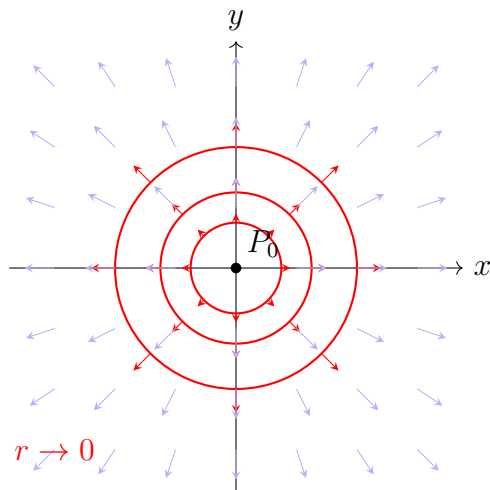
Figure 5.21: As we shrink our test curve around P_0 , we measure the local expansive tendency of the field. The normal vectors (red) measure outward flow at each point.
