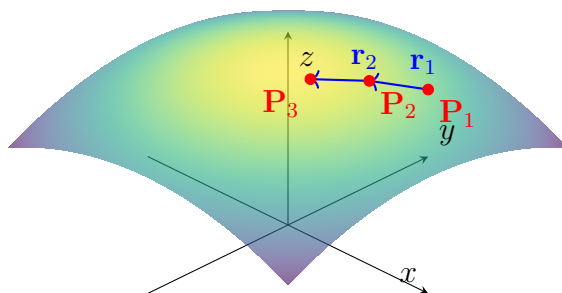
Figure 3.18: The gradient ascent of the two vectors found in this problem starting at point \mathbf{P}_1 = (0.5, 0.5) .
