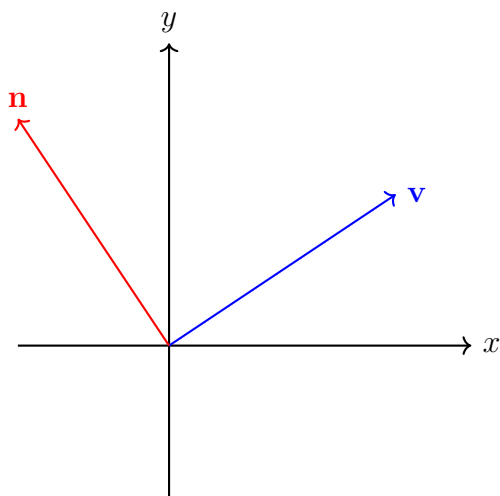
(a) Normal vector in Cartesian coordinates
