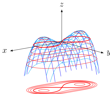
Figure 3.4: A 3D surface featuring with its level curves shown below featuring the Bernoulli lemniscate (the infinity shaped level curve)
