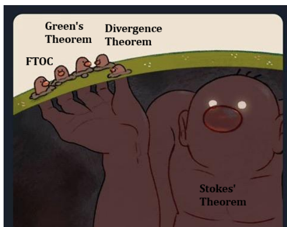
Figure 5.31: The master of all: Stokes' Theorem
