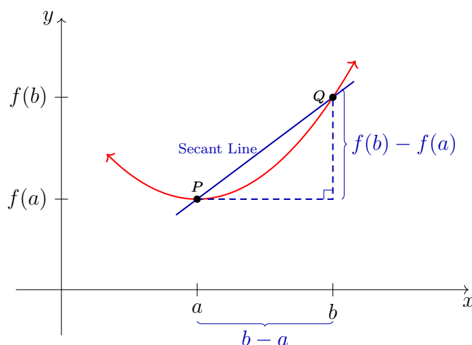
Figure 1.2: A secant line threading two points along a curve f(x) .
