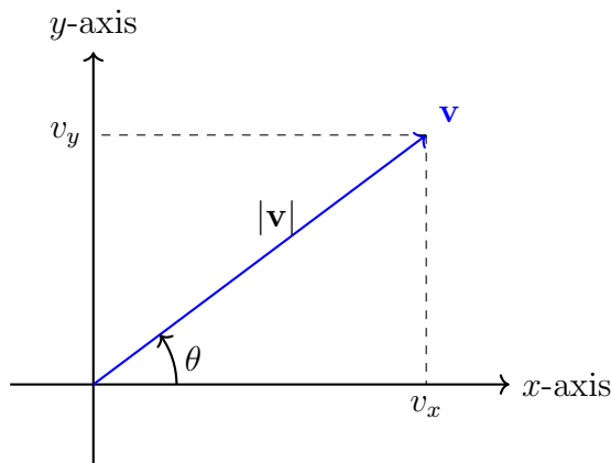
Figure 1.13: A 2D vector \mathbf{v} showing the angle \theta with the x -axis. The direction cosine, \cos \theta , is the ratio \frac{v_x}{|\mathbf{v}|} , which describes the vector's orientation relative to the x -axis.
