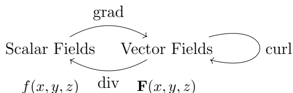
Figure 5.24: The relationships between vector operators. Gradient maps scalar to vector fields, divergence does the reverse, and curl maps vector fields to vector fields.
