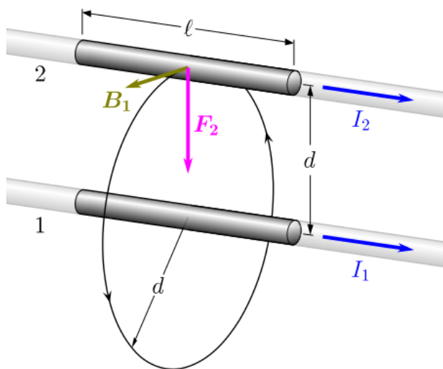
Figure 5.30: This image shows the magnetic force F_2 between two parallel current-carrying wires. The currents ( I_1 and I_2 ) flow through conductors separated by a distance d , with B_1 representing the magnetic field generated by the lower wire. The conductors have length \ell , illustrating the Ampère-force law and how parallel currents create magnetic fields that interact with each other.
