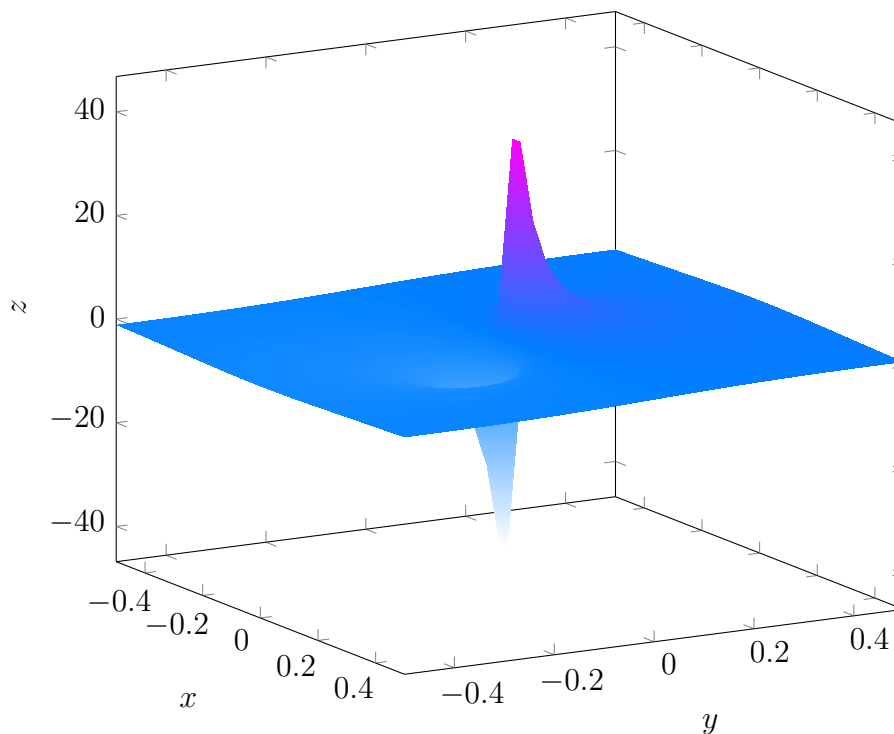
Figure 4.4: A plot of the function f(x, y) = \frac{y}{x^2 + y^2} . Notice that the function is odd, and thus integrating across symmetric bounds produces volume equal to 0.
