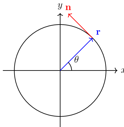
(b) Normal vector on a circle (polar)
