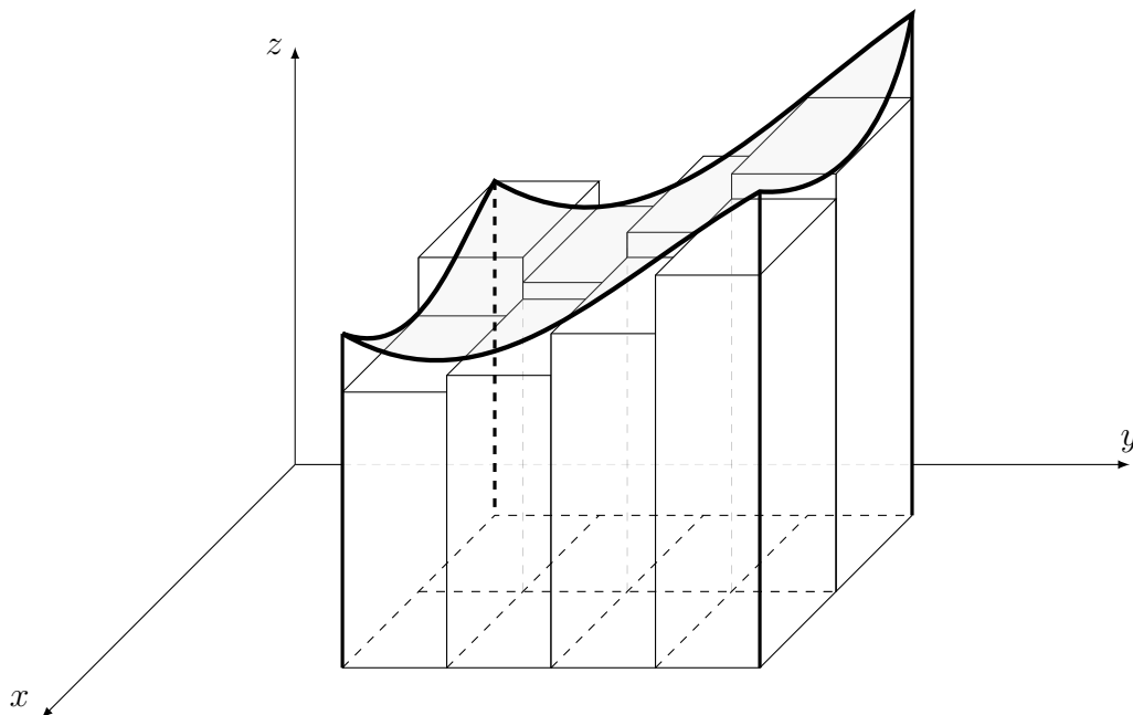
Figure 4.2: The Riemann Sum approximation of the volume under a curve. When taking the limit of these rectangular prisms to be infinitesimally small, we approximate the double integral.
