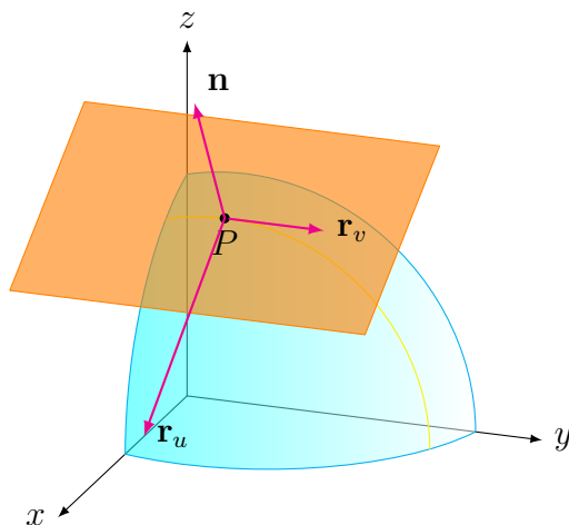
Figure 5.26: At each point P on the surface, the vectors \mathbf{r}_u and \mathbf{r}_v span the tangent plane, while their cross product \mathbf{n} gives the normal direction.
