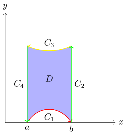
Figure 5.12: A region D bounded by a curve C = C_1 + C_2 + C_3 + C_4 . We can begin to heuristically see the relationship between the line integral and the volume double integral.
