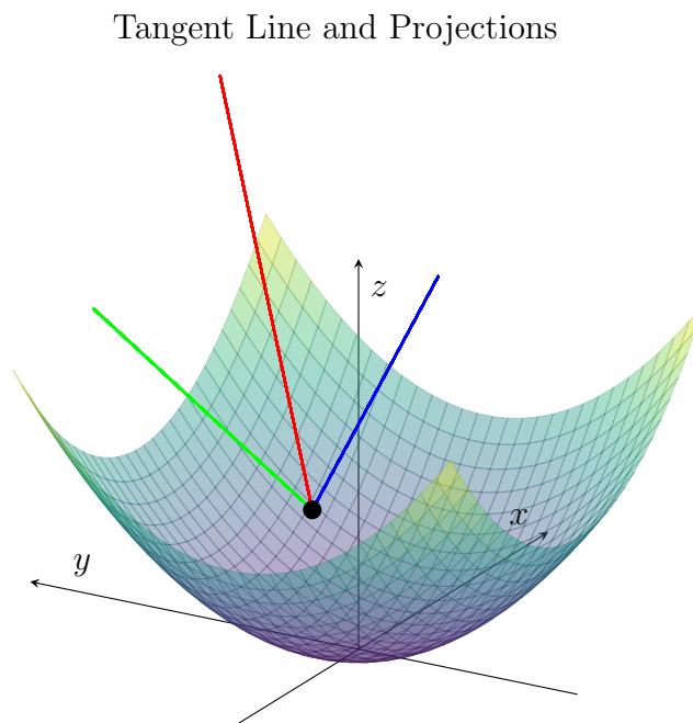
Figure 3.14: Derivative of a surface z = x^2 + y^2 at a point (1, 1, 2) . The tangent line (red) is notated with projections of each component, green indicating yz -plane projection of the tangent line, and blue indicating the xz -plane projection.
