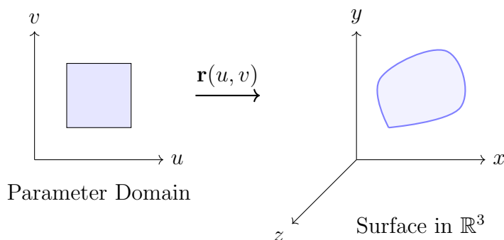
Figure 5.25: The parametric mapping \mathbf{r}(u, v) transforms regions in the parameter plane to pieces of surface in three-dimensional space.
