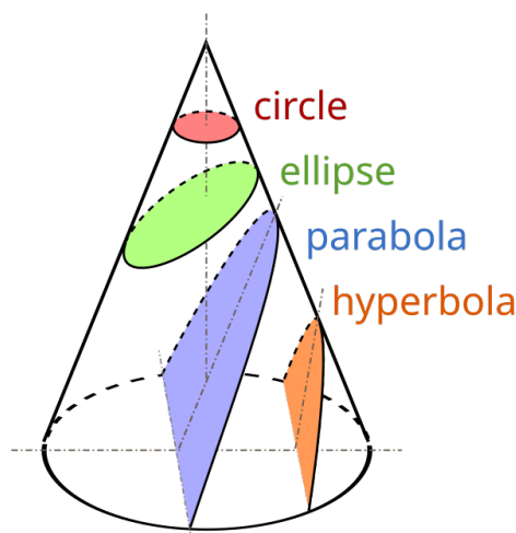
Figure 1.27: Conic sections derived from a single-napped cone. The hyperbola includes an additional section, as the intersecting plane extends through the origin to cut both nappes of the cone when there are two present.
