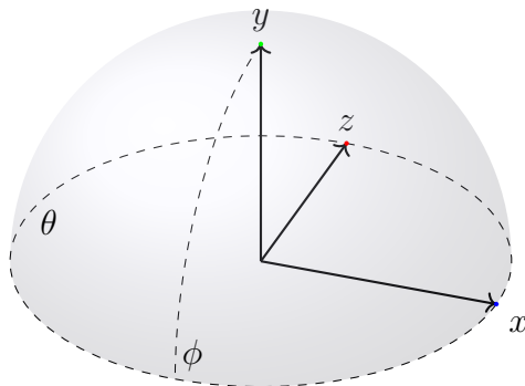
Figure 5.27: The hemispherical dome with spherical coordinates (\phi, \theta) shown.
