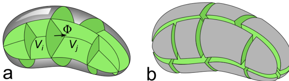
Figure 5.32: (a) Adjacent subvolumes V_i and V_j sharing an interface \Phi through which the field flows. (b) Complete subdivision of a volume showing all interfaces (green). Interior interfaces cancel in pairs, leaving only boundary contributions.
