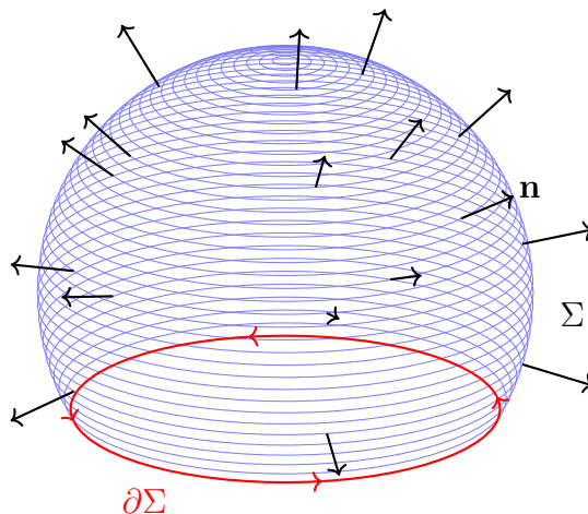
Figure 5.29: Visualization of Stokes' Theorem: a portion of the unit sphere \Sigma emerging from a fluid with outward-pointing normals \mathbf{n} . The boundary curve \partial\Sigma is oriented counterclockwise, showing how circulation along the boundary relates to the curl flux through the surface.
