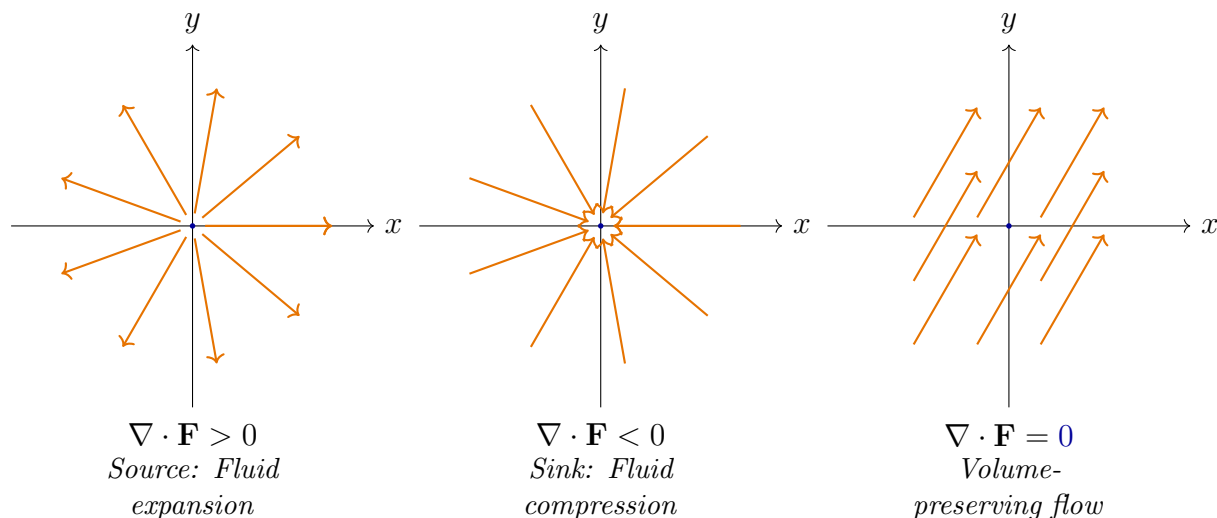
Figure 5.22: Fundamental divergence patterns in vector fields. The divergence measures the net flux per unit area. Left: A source field exhibits positive divergence as vectors emanate outward, indicating fluid expansion. Center: A sink field shows negative divergence as vectors converge inward, representing compression. Right: An incompressible flow field maintains zero divergence, preserving volume as fluid moves. Note how the vector patterns visually represent the mathematical concept of divergence through their geometric arrangement.
