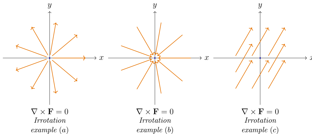
Figure 5.19: Vector field patterns that have 0 curl. The arrows clearly show no local rotation about the point.
